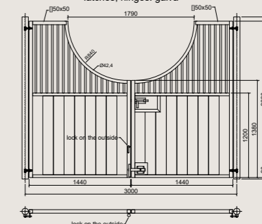
F07DEARG320/CF2463 - 1 pcs RESINE GRAY 32mm, GALVA latches, hinges: galva
